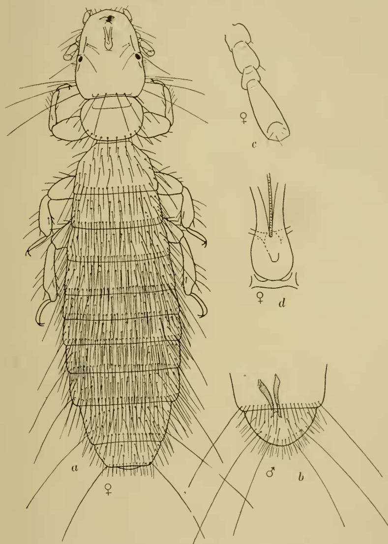
FIG. 1.— Somaphantus lusus , Paine. a , female; b , last segments of male; c , antenna of female; d , pharyngeal sclerite of female.
